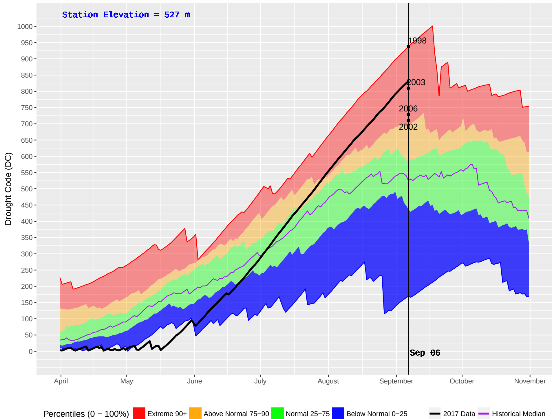
SALMON ARM (346) : Historical (1976–2016) and Current (2017) Noon Drought Code (DC)
