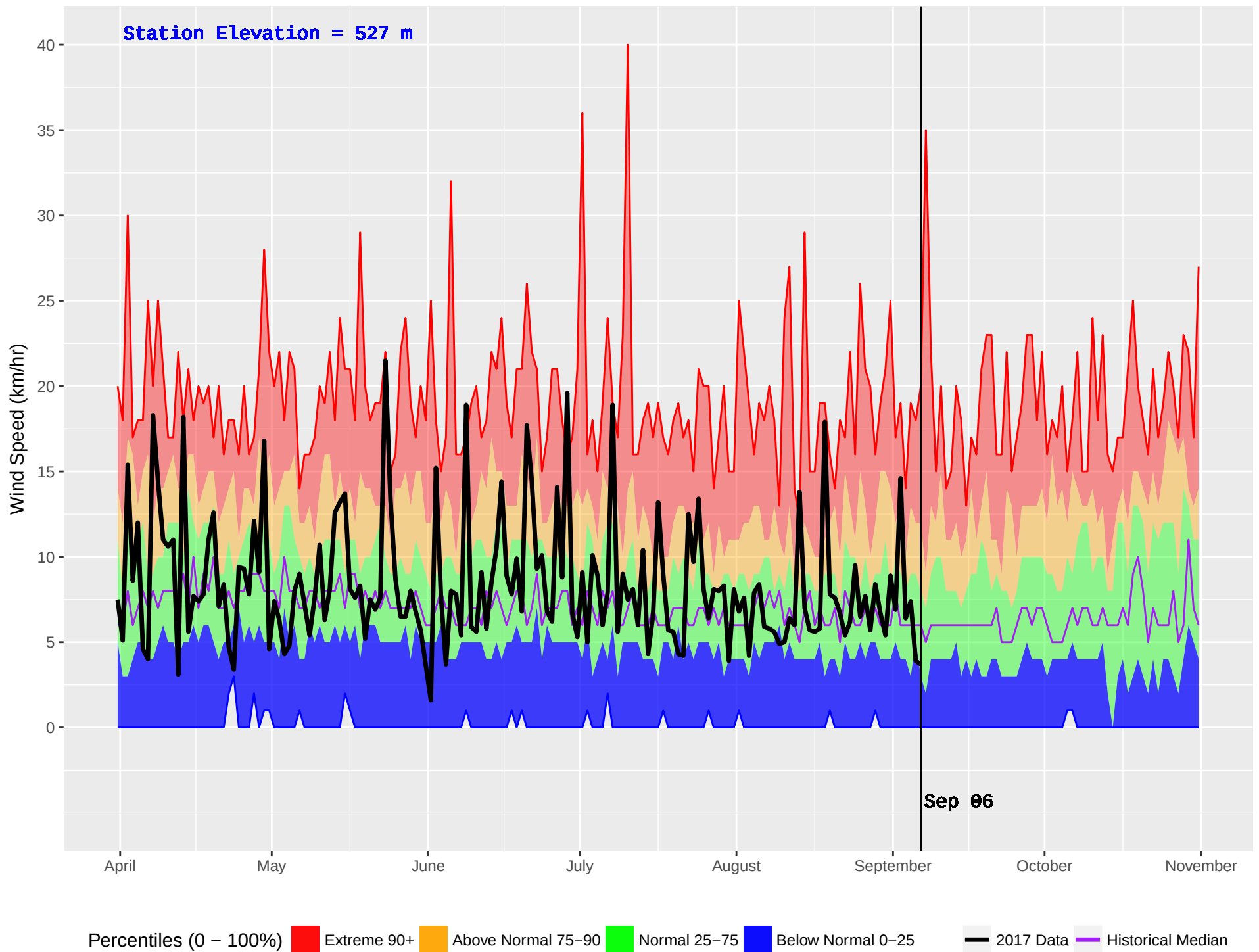
SALMON ARM (346) : Historical (1976–2016) and Current (2017) Noon Wind Speed
